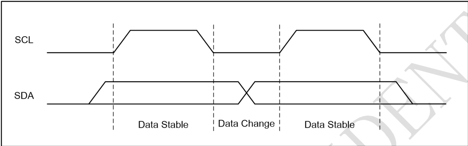
Figure 4-1 Data Validity
