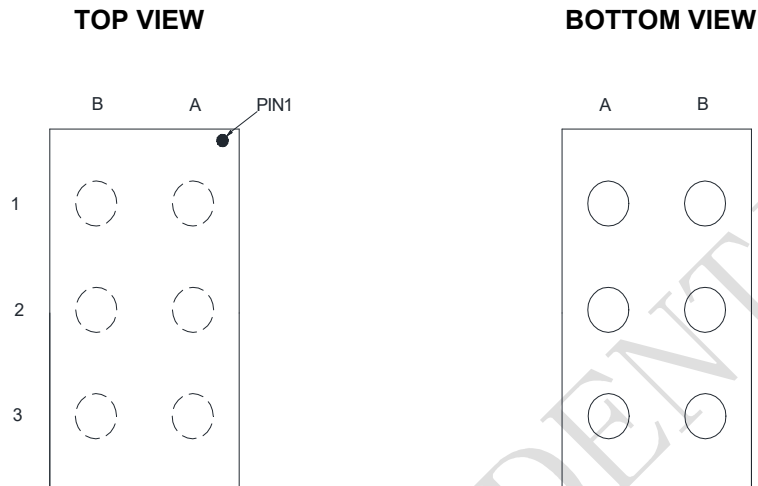
Figure 1-1 WLCSP6 (Ball pitch 350um*350um)
