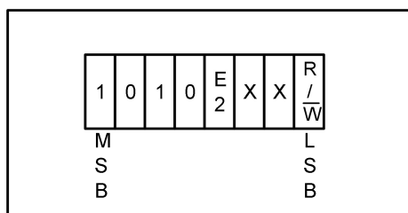
Figure 4-5 Device Address
