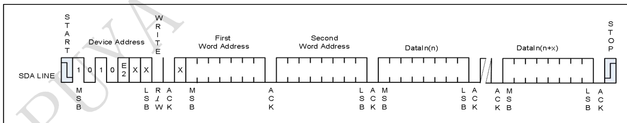
Figure 5-2 Page Write
