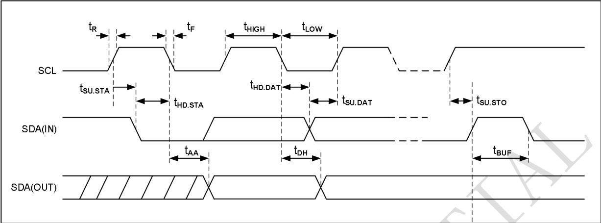
Figure 3-1 Bus Timing
